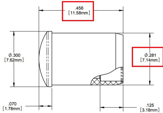
CML_327_CTP - Incorrect Dimensions (Old Datasheet):
