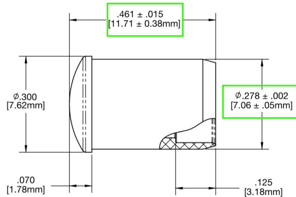
CML_327_CTP - Correct Dimensions (New Datasheet):
